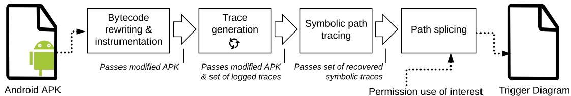
Fig. 2: Hogarth’s architecture.
